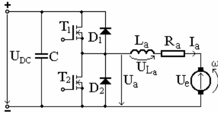
Fig. 2 Half bridge chopper circuit
